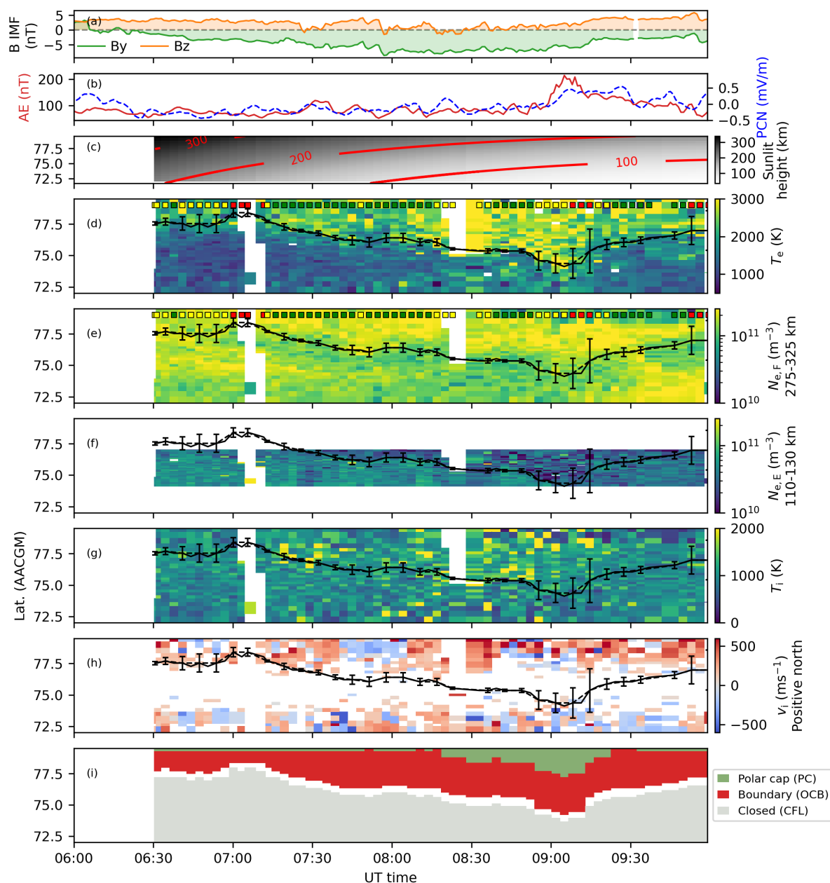
Figure 2. Overview of observed T_e , T_i , v_i and N_e , and identified regions on open and closed field lines by the ESR 32 meter from December 4 2014. Panel a shows the IMF B_z and B_y components, panel b the AE (red solid, left hand axis) and PCN (blue dashed, right hand axis) indices, (c) the lowest altitude that is illuminated, panels (d, e, f, g, h) show T_e , N_{e,F} (high F-region (275-325 km), N_{e,E} (E-region, 110-130 km), T_i and v_i observed at 300 km altitude by the 32 meter along the geographic meridian. The solid black line indicates the open-closed field line boundary. The colored squares show the quality flags. Panel i shows colored regions of the 32-meter data corresponding to closed field lines (grey), in the polar cap (green) and along the open-closed field line boundary (red).
