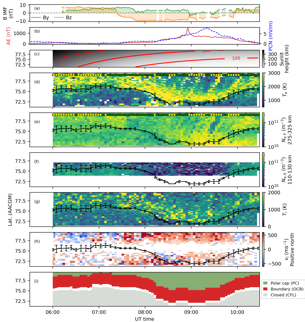
Figure 3. Same as Fig. 2 for December 5 2015.
